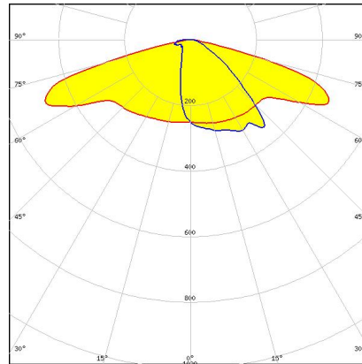
CS16397_STRADA-IP-2X6-T2-C-90-PC CS14145_STRADA-IP-2X6-DWC-90
