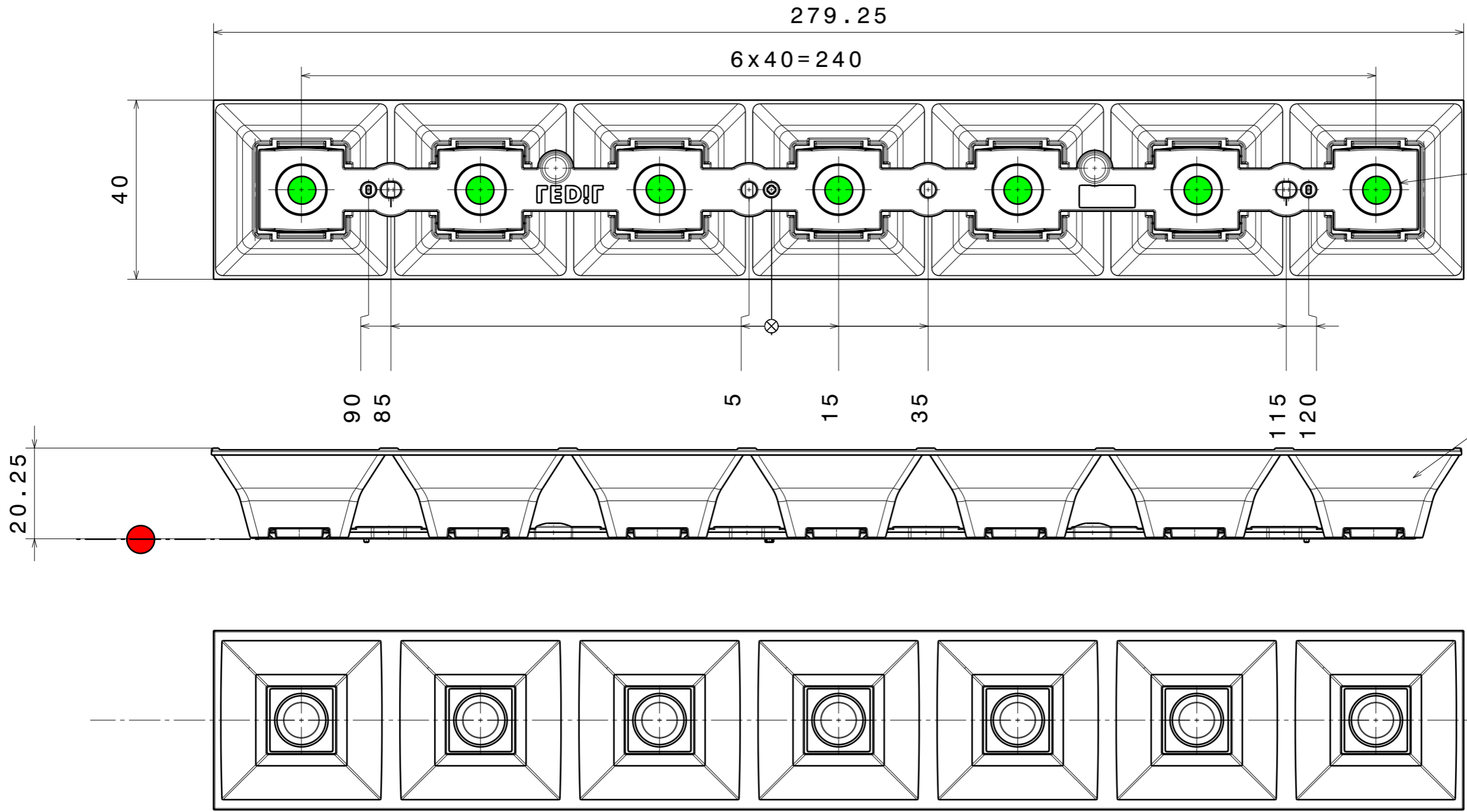
CN16873_DAISSY-7x1-WW_Mechanical Model
