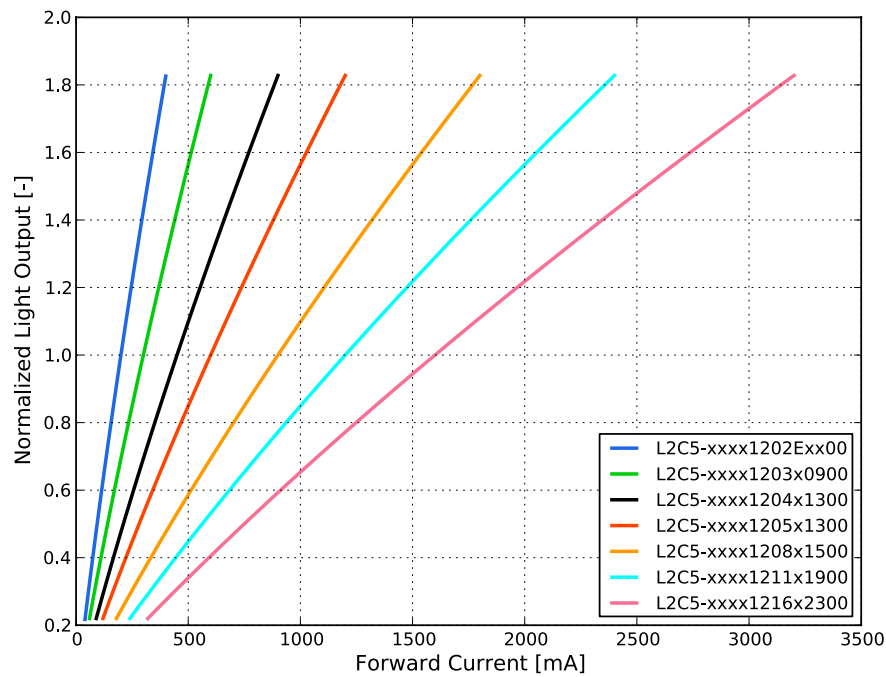
Figure 3a. Typical normalized light output vs. forward current for L2C5-xxxx12xxxxx00 at T j =85°C.
