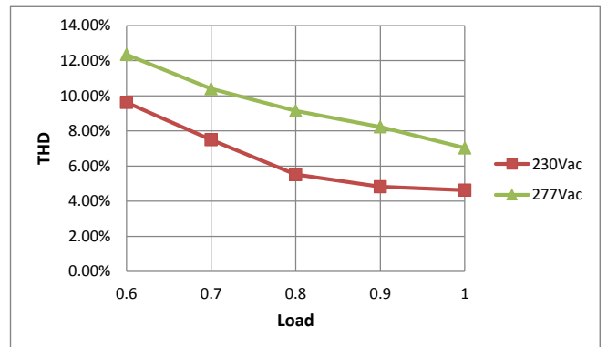
THD Curve
